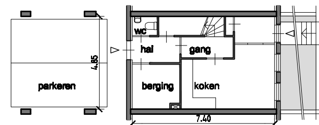
1:200, begane grond
